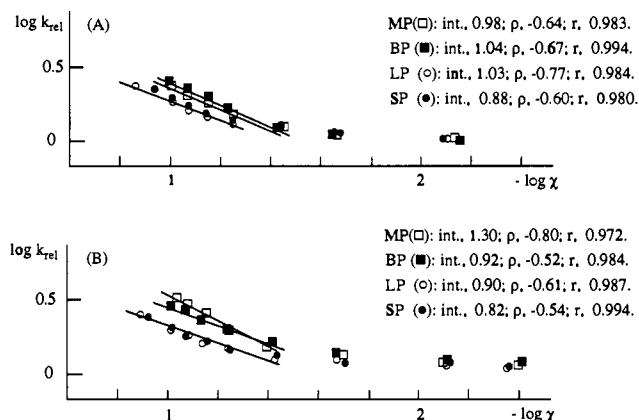
Figure 4. (A) Plot of log k_{rel} vs -\log \chi for the DA reaction of 7 and 8 at 20 °C in the presence of the different perchlorates (Table III). (B) Same for the DA reaction of 1 and 10 at 20 °C (Table IV). The regression data for each linear relationship are calculated with the starred values in Tables III and IV.
