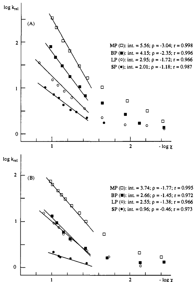
Figure 3. (A) Plot of \log k_{rel} vs -\log \chi for the DA reaction of 1 and 2 at 30 °C in the presence of the different perchlorates (Table I). (B) Same for the HDA reaction of 4 at 20 °C (Table II). The regression data for each linear relationship are calculated with the starred values in Tables I and II.
